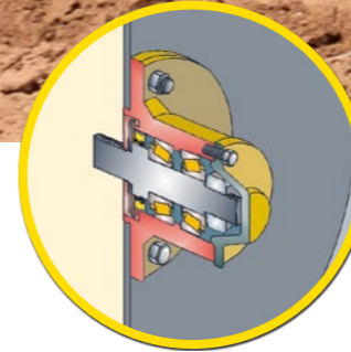
1 15"X15" UNALIGNED DOUBLE DISCS WITH TWO BALL BEARINGS ON EACH HUB ARE SUPPLIED FOR FERTILIZER AND SEEDS.
